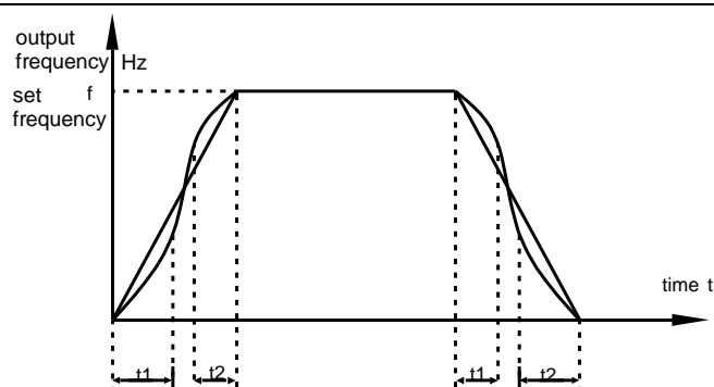
Graph4-11 S-curve acceleration/deceleration A
