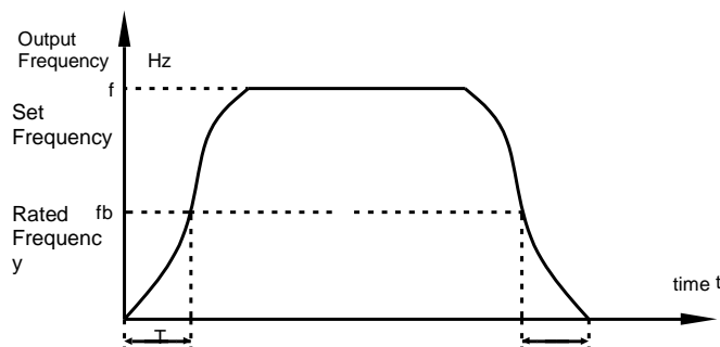
Graph4-12 S-curve acceleration/deceleration B
